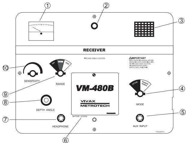
VM-480B Receiver: Controls and Indicators
