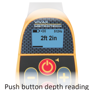
Peak locate response with accompanying audio tone
